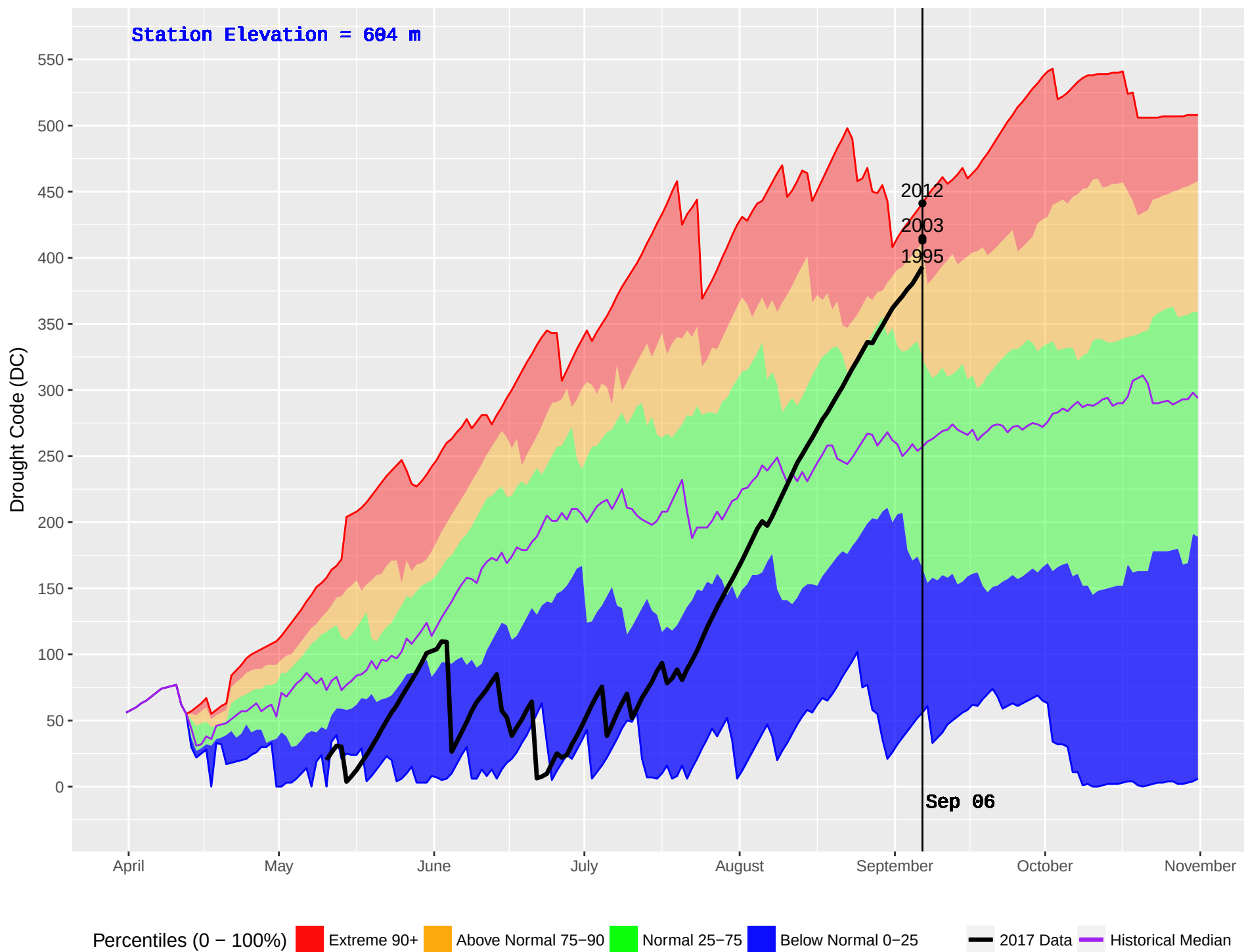
NELSON FORKS (119) : Historical (1986–2016) and Current (2017) Noon Drought Code (DC)
