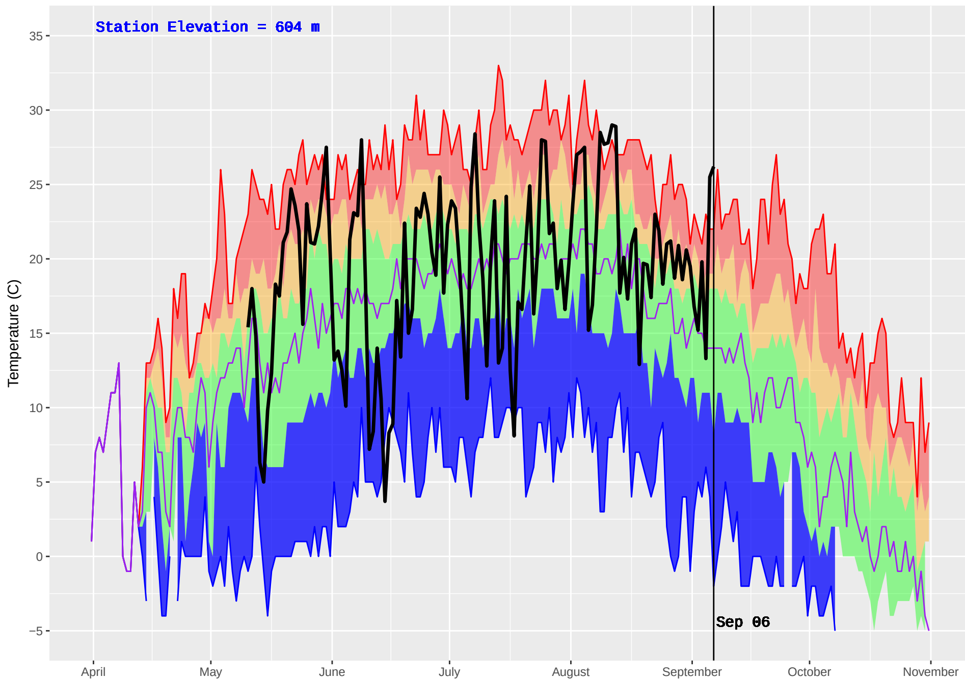
NELSON FORKS (119) : Historical (1986–2016) and Current (2017) Noon Temperature
